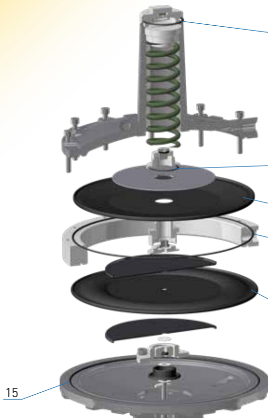
RS 250 / 251 shown with safety diaphragm (version 1)
