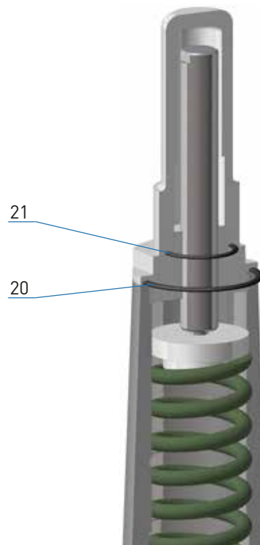
RS 250 / 251 shown with HDS high-pressure screw spindle
