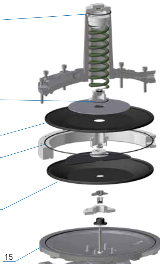
RS 250 / 251 shown with safety diaphragm (version 2)
